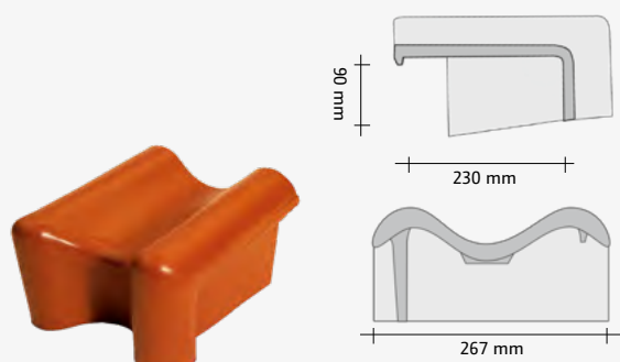
Pulldach-Giebelortgangziegel, links Chaperon gevelpan links · Tuile de rive shed gauche
