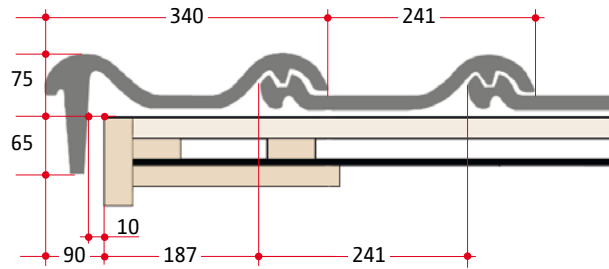
Maße Ortgang links
